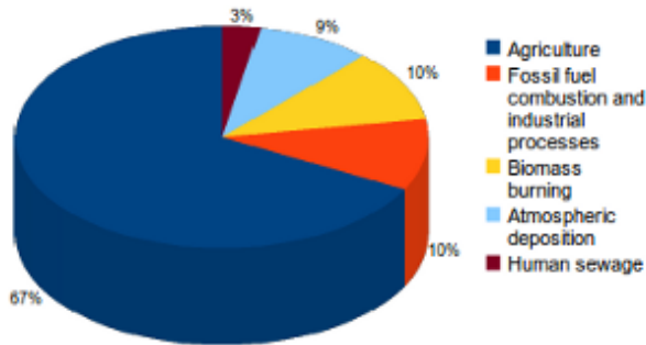
Human sources of nitrous oxide
