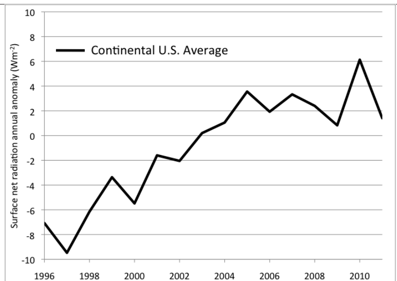
Fig. 5 The change in net radiation at the surface derived for continental U.S. over 15 years of SURFRAD measurements. This increase is mostly in the shortwave and is likely associated with reduced cloud cover.
