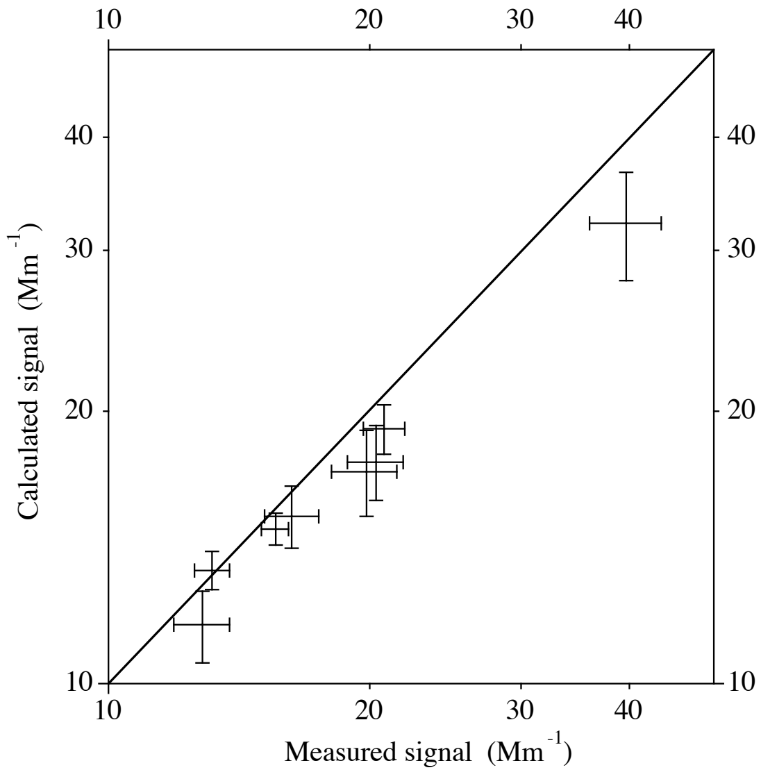
Figure 1k As Figure 1h but for TSI blue back-scatter signals.
