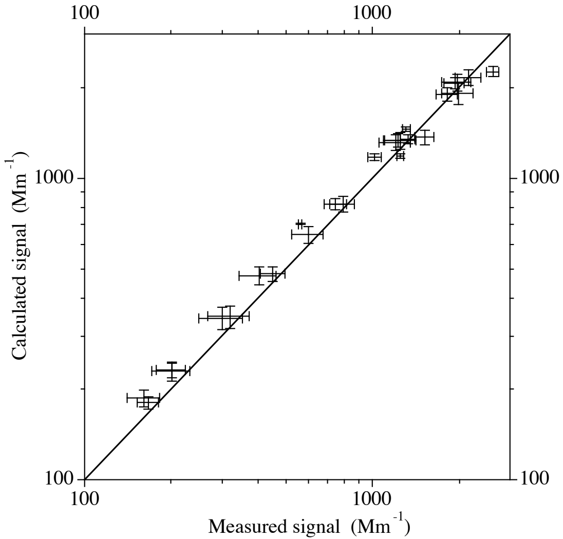
Figure 1b As Figure 1a but for TSI green total scatter signals.
