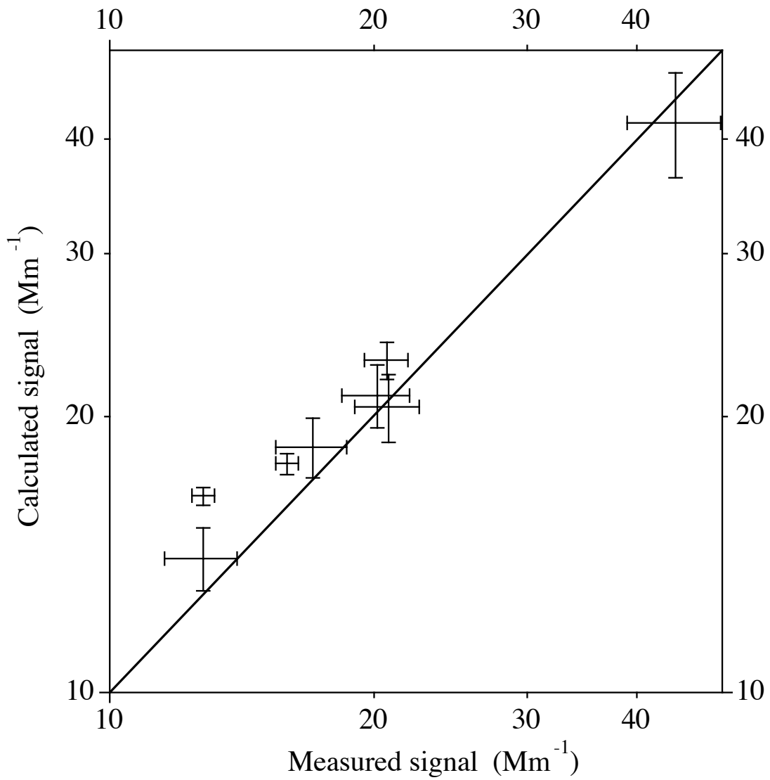
Figure 11 As Figure 1h but for TSI green back-scatter signals.
