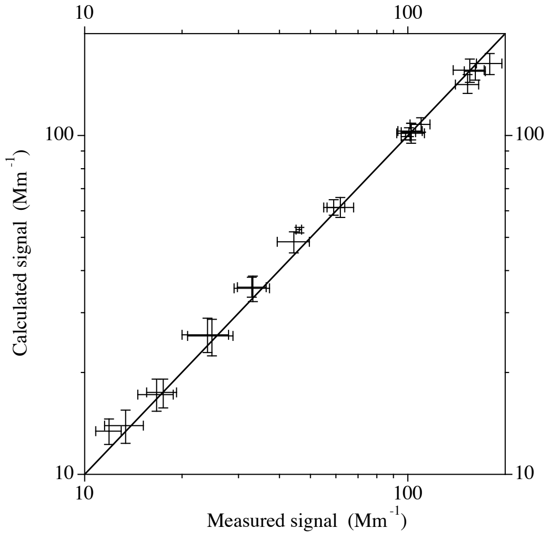
Figure 1e As Figure 1a but for TSI green back-scatter signals.
