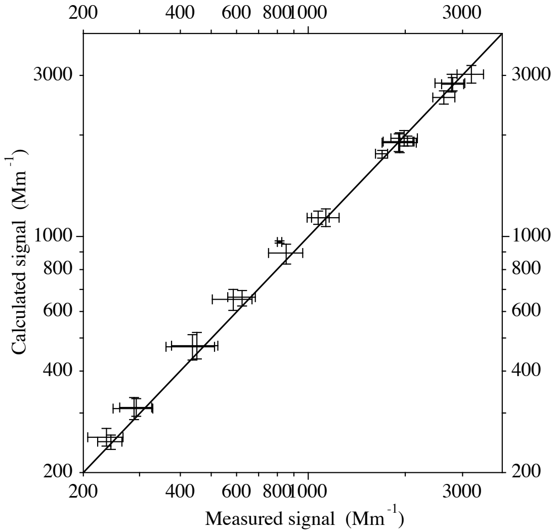
Figure 1a Scatter-plot of average measured and Mie-calculated nephelometer total scatter signals for sub-micrometer test aerosols and TSI blue signals. Error bars indicate the uncertainties of measured and calculated signals.
