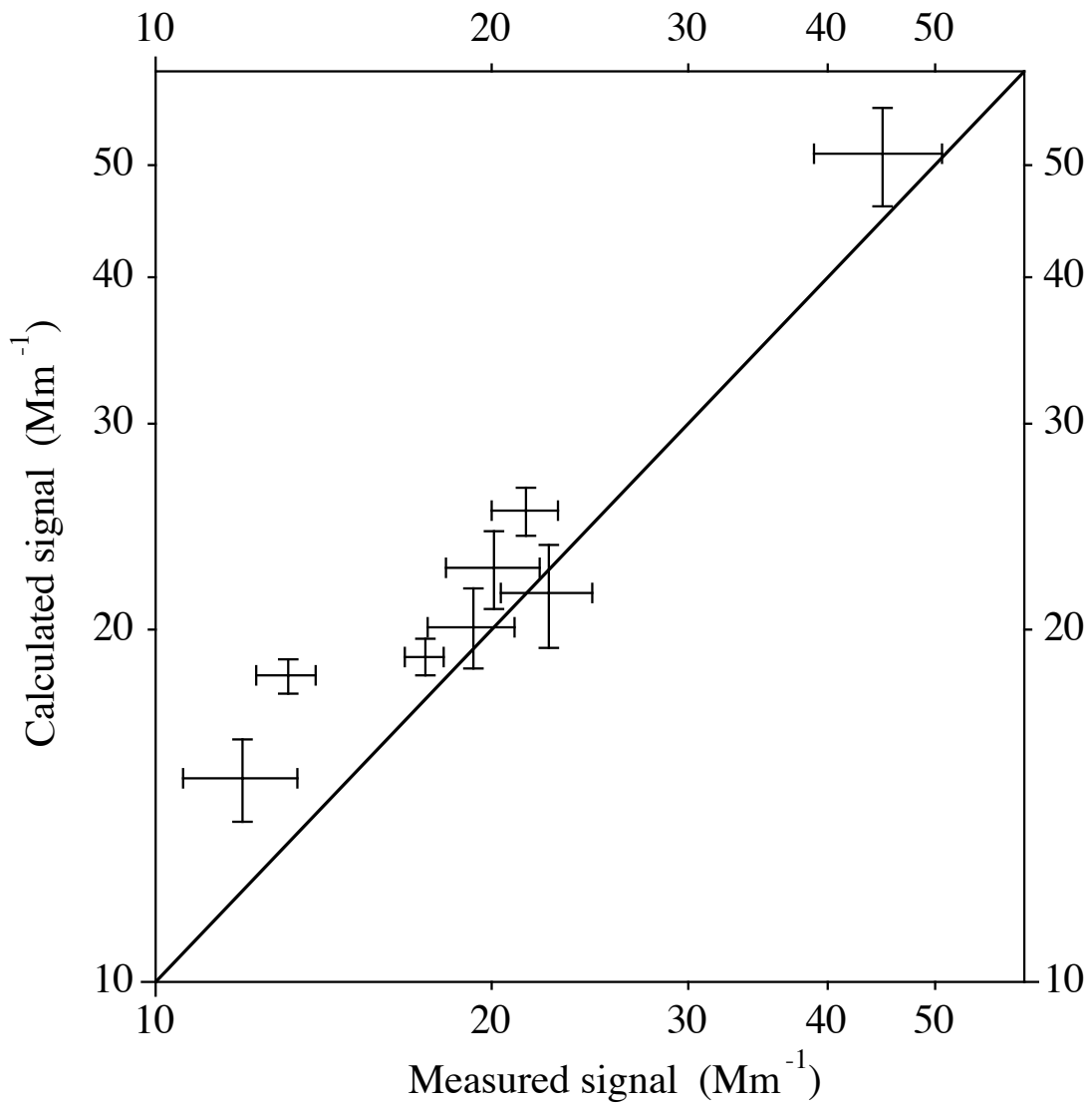
Figure 1m As Figure 1h but for TSI red back-scatter signals.
