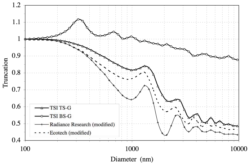
Figure 3 Theoretical size-dependent signal truncations for DEHS aerosols with the average size distribution of the present study and the green total (TSI TS-G) and back-scatter (TSI BS-G) channels in the TSI nephelometers, the empirically modified angular sensitivities of Radiance Research and Ecotech nephelometers. The truncations are normalized by the Rayleigh-truncation to reflect the result of a gas calibration.
