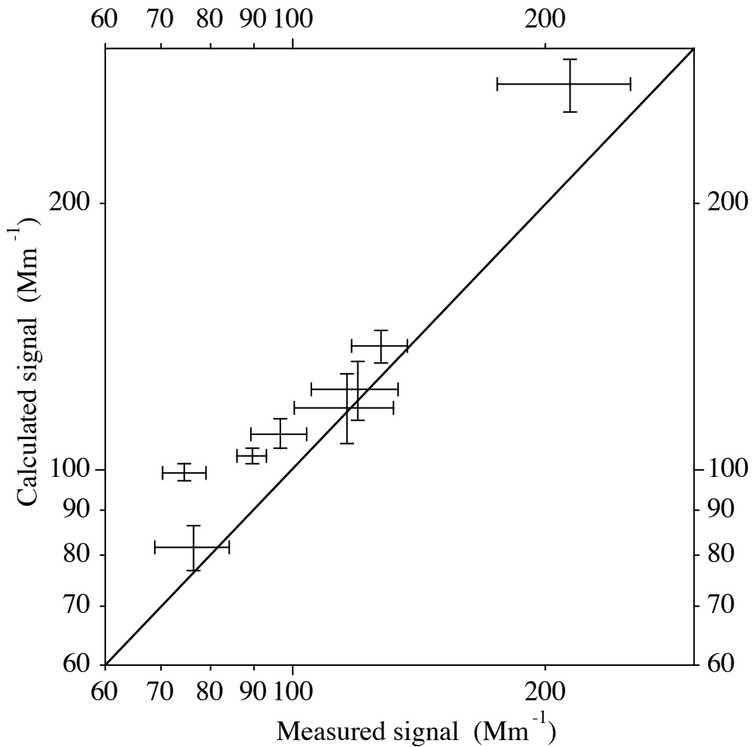
Figure 1h Scatter-plot of average measured and Mie-calculated nephelometer total scatter signals for super-micrometer test aerosols and TSI blue signals. Error bars indicate the uncertainties of measured and calculated signals.
