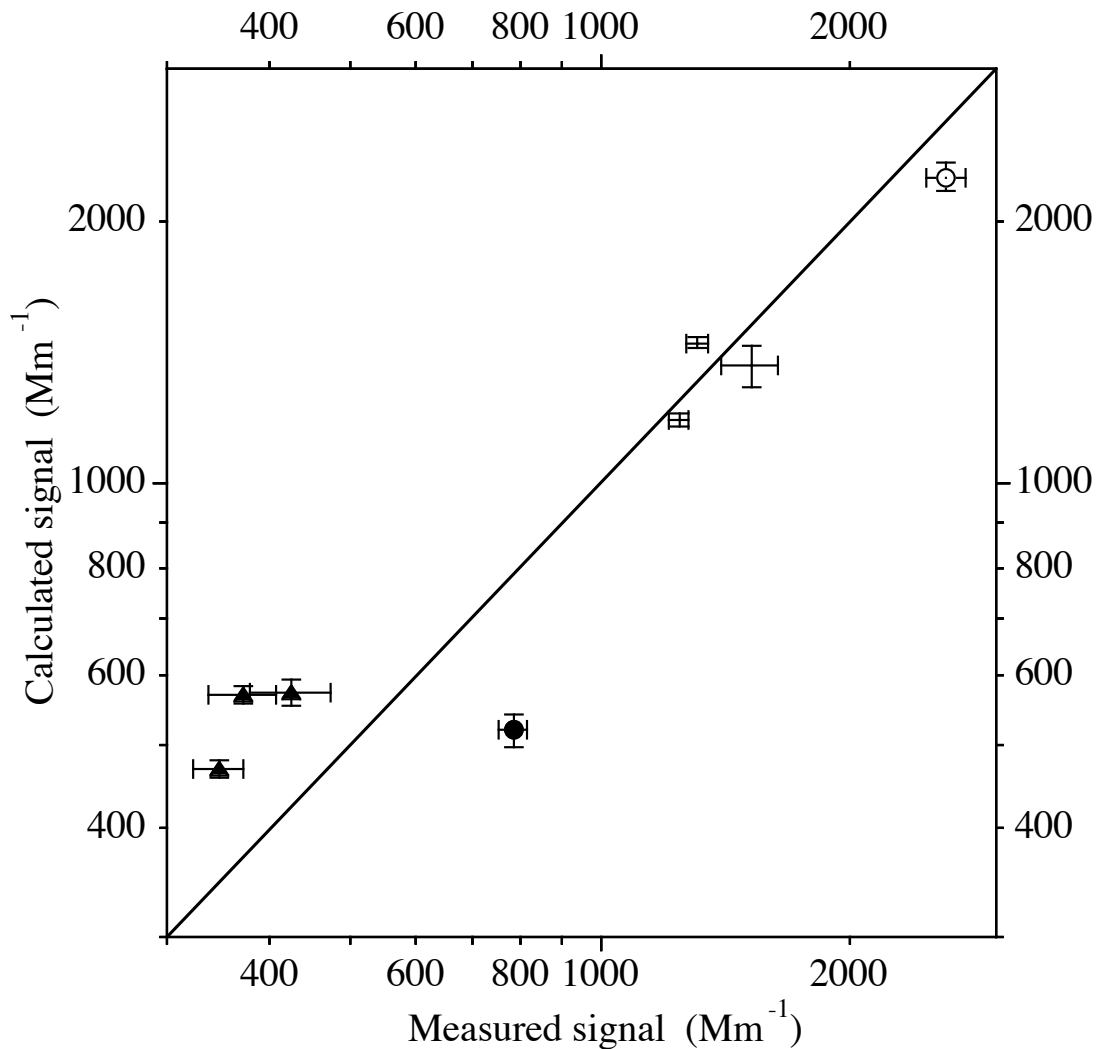
Figure 1g Scatter-plot of average measured and Mie-calculated nephelometer total scatter signals for Radiance Research sub-micrometer (cross) and super-micrometer (full triangle) signals and for Ecotech sub-micrometer (open circle) and super-micrometer (full circle) signals. Error bars indicate the uncertainties of measured and calculated signals.
