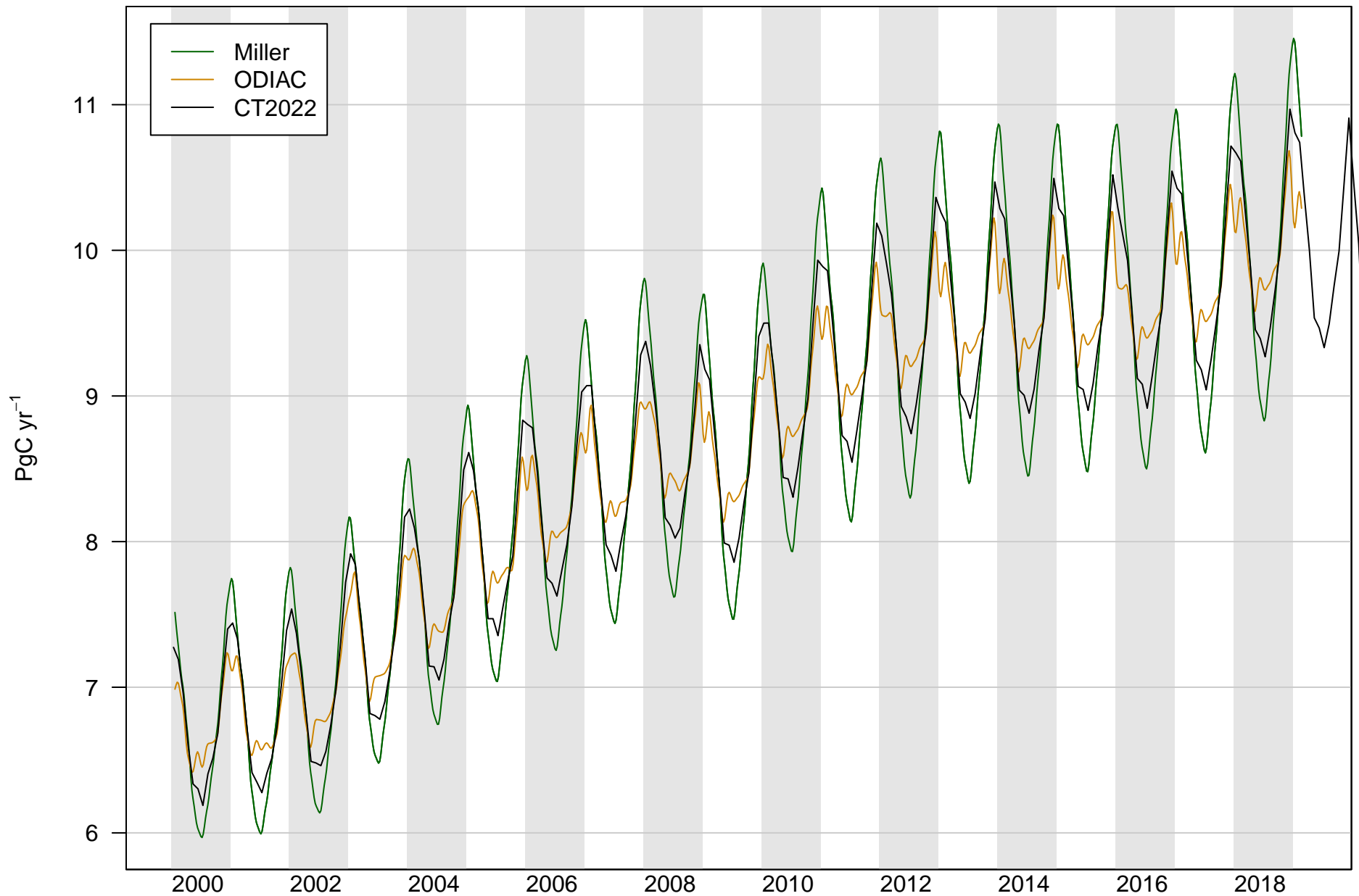
Global total fossil fuel emissions
